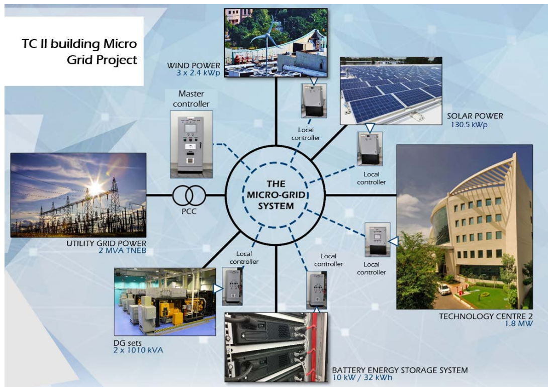
Figure 23: L&T Chennai Campus Technology Centre II Microgrid Features
