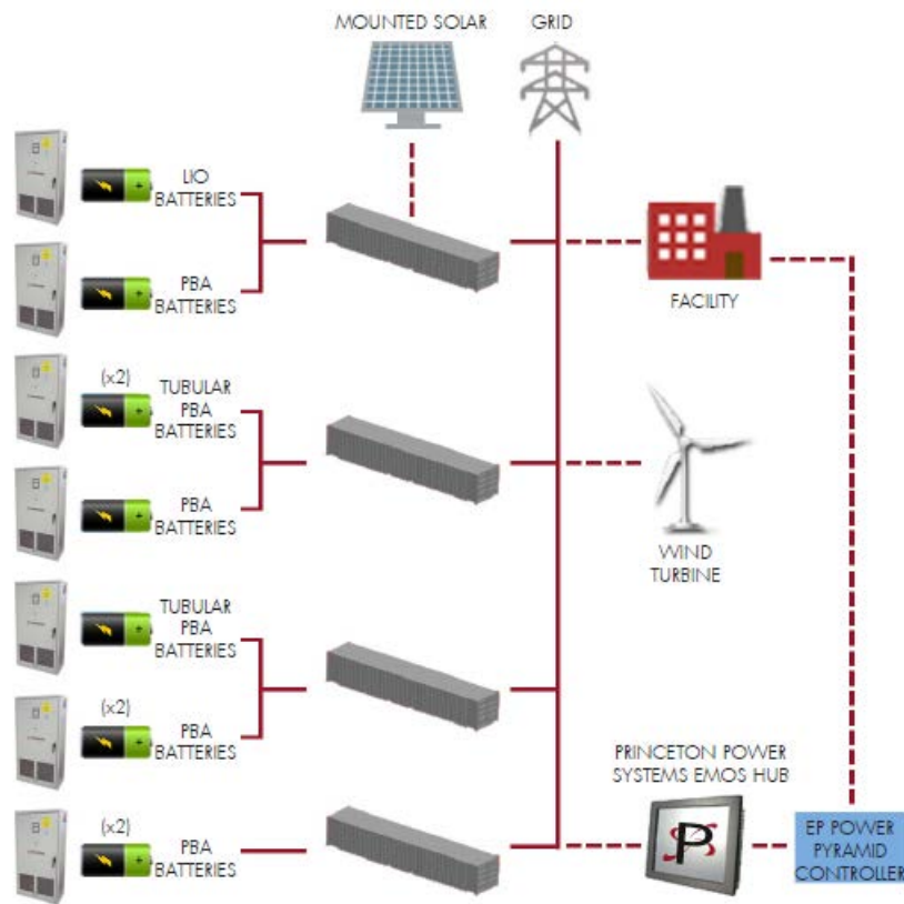
Figure 14: EaglePicher Power Pyramid™ Diagram Featuring Three Battery Technologies
