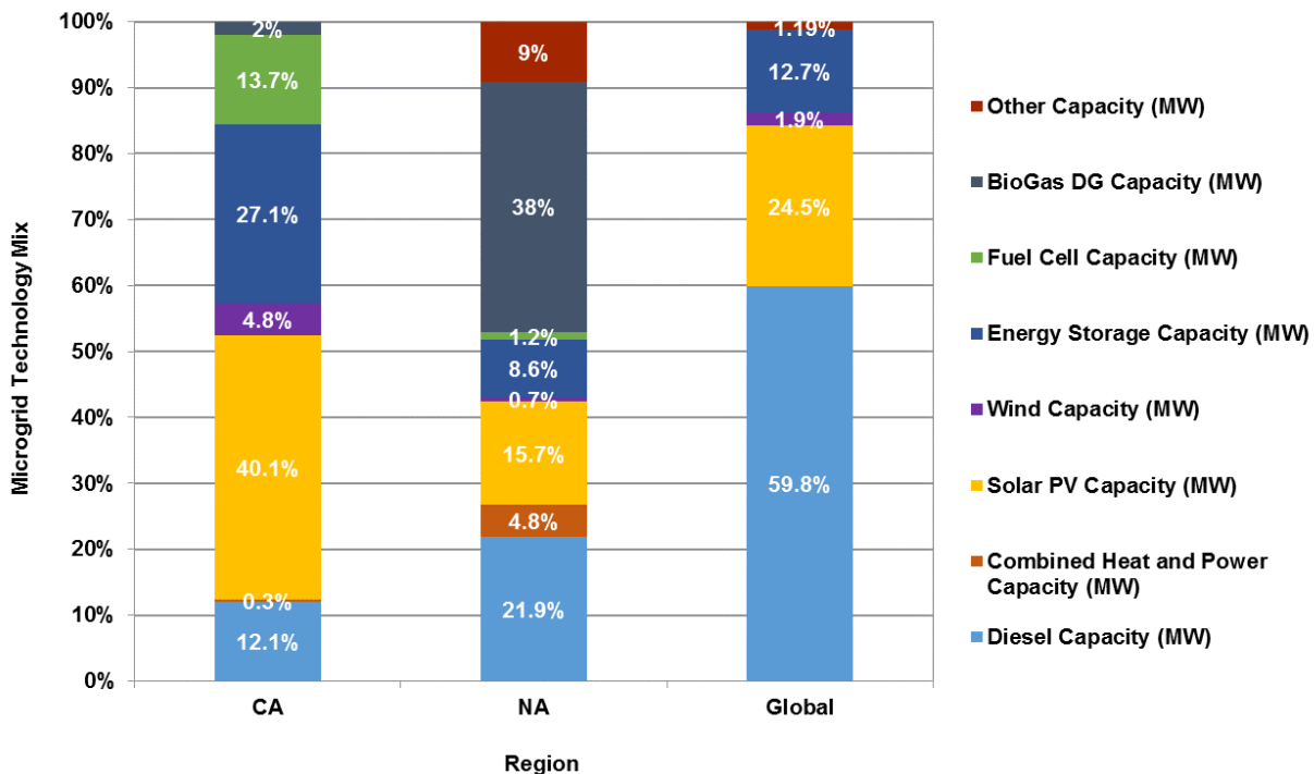
Figure ES-5: Comparison of DER Mix, by Region
